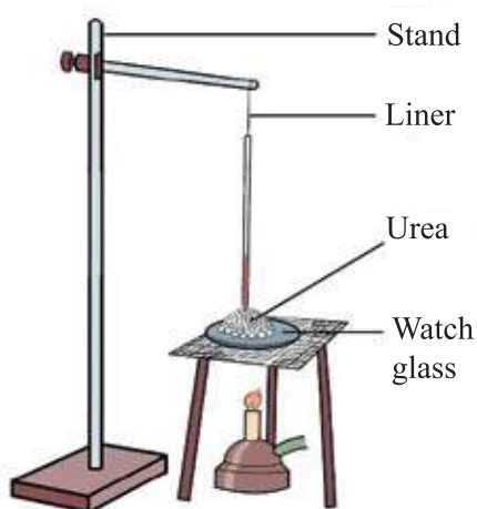
Fig 2.06: Melting point of urea.
