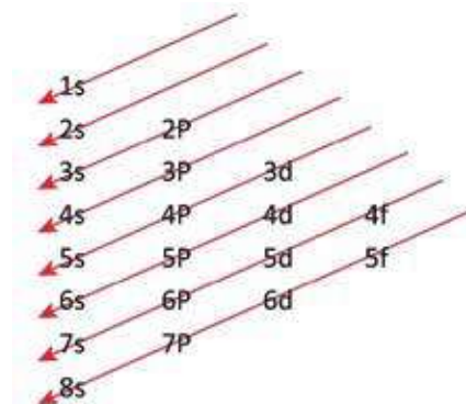
Fig 3.04: Sequence of Energy of Orbitals.
