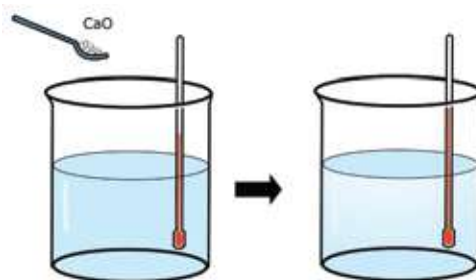
Fig 8.18: Solution of lime in beaker.
