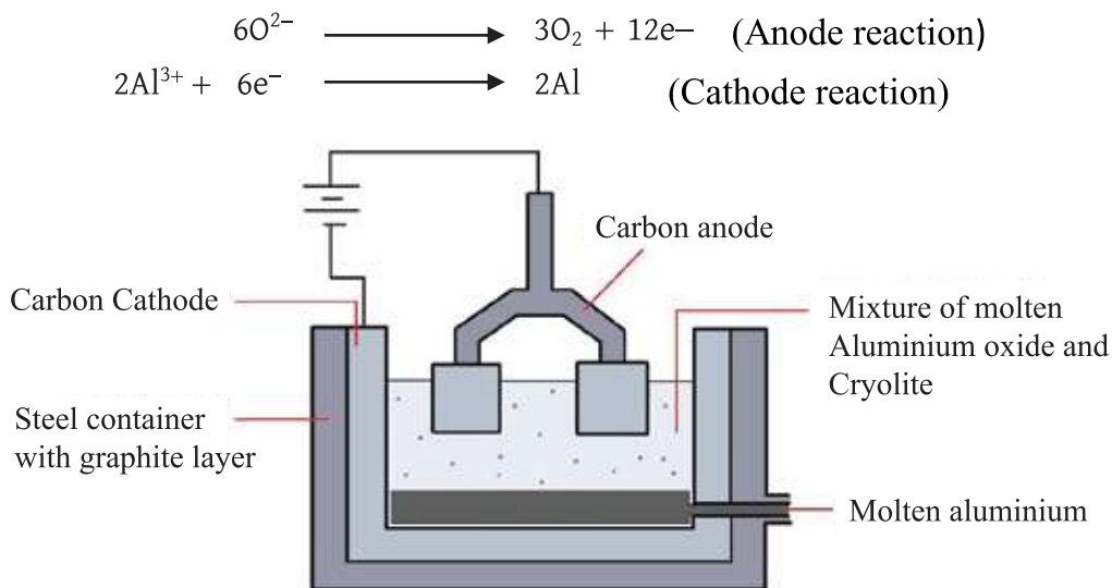
Fig10.07: Aluminium Extraction.
