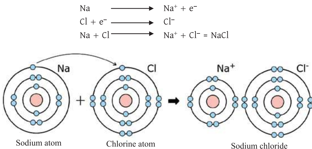
Fig 5.06: Formation of sodium chloride.
