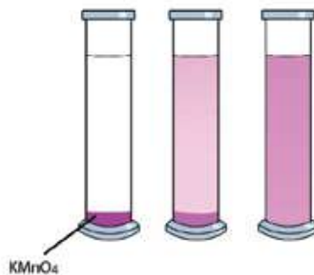
Fig 2.02: \text{KMnO}_4 solution in water.
