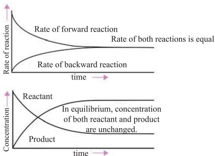
Fig 7.05: Chemical equilibrium.
