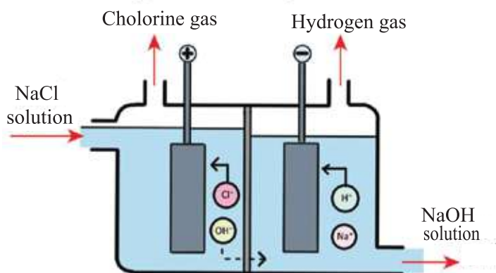
Fig 8.05: Electrolysis of Sodium Chloride Concentrate Solution.
