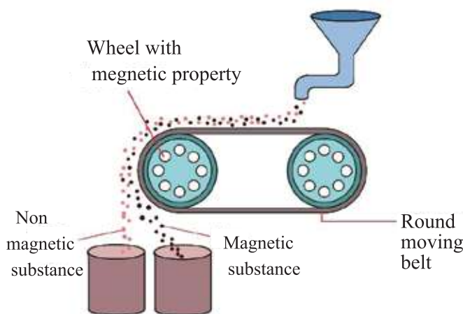
Fig 10.06: Magnetic Separation.
