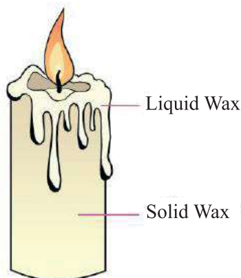
Fig 2.05: Burning of Wax.
