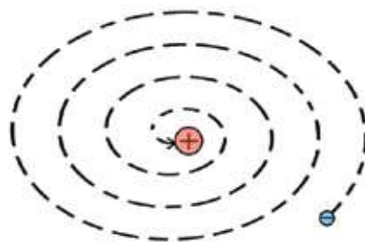
Fig 3.02: Electron falling on nucleus.
